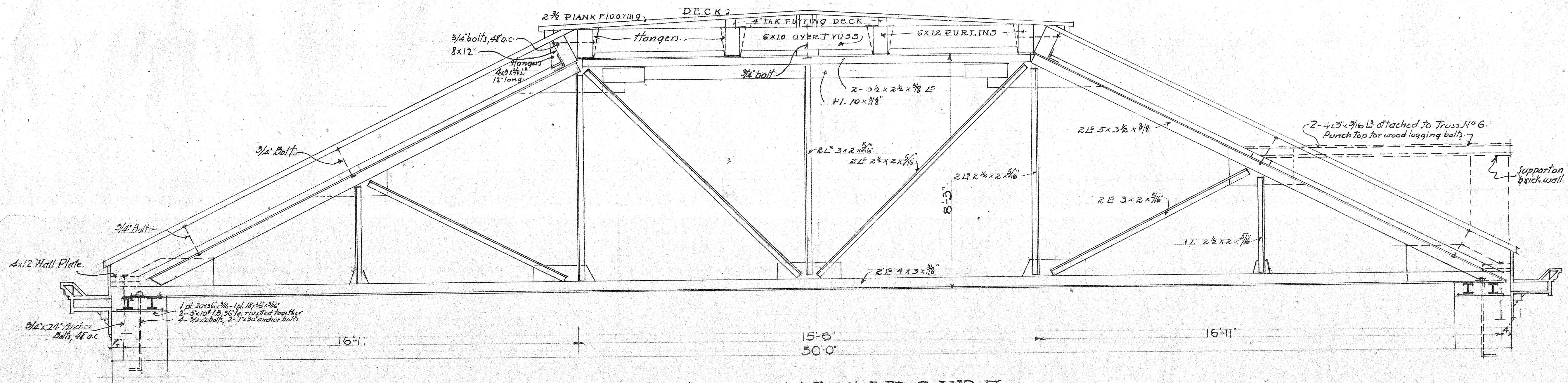
DETAILS OF TRUSSES NO 6 AND 7.
