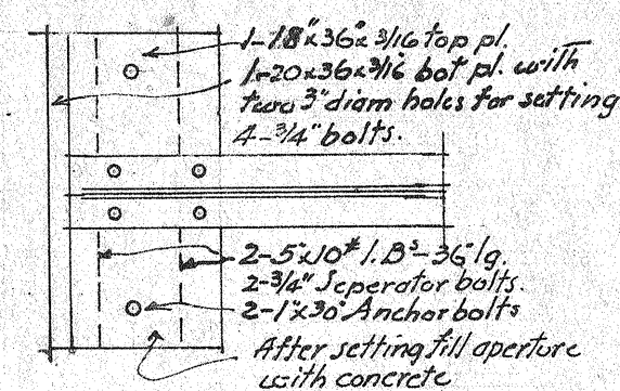
DETAIL OF BED PLATE.
